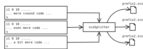
Figure 2: Splitting the score
